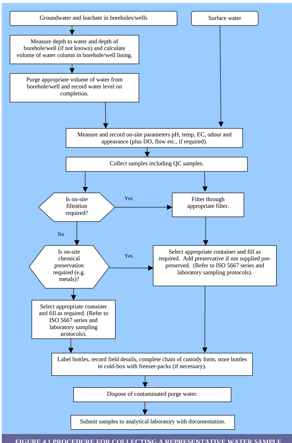
FIGURE 4.1 PROCEDURE FOR COLLECTING A REPRESENTATIVE WATER SAMPLE
